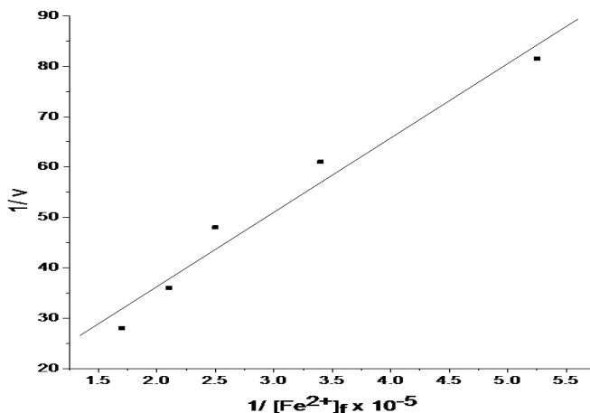
Figure 1: Plot of 1/v versus 1/[Fe^{2+}]_f as a Function of 0.50 \times 10^{-4} \text{ mol dm}^{-3} \text{ H}^+ of Binding between Fe(Me_4phen)_3^{2+} and SDS
